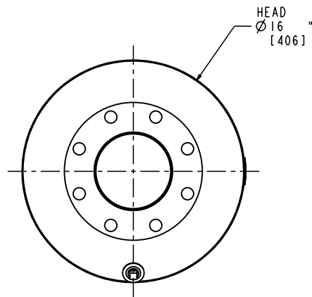
VIEW FROM INLET END
