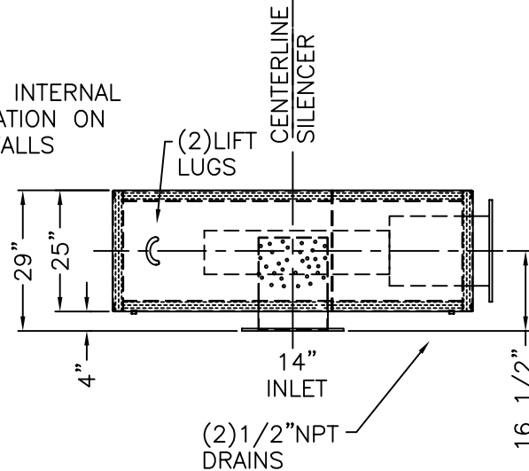
14" OUTLET SIDE VIEW
